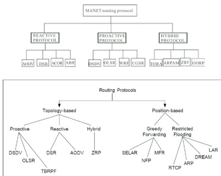
FIG.1 Routing protocols in MANET
