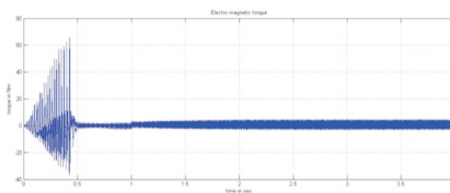
Fig.13. Generated torque of the 5-level proposed multilevel inverter fed BLDC motor
