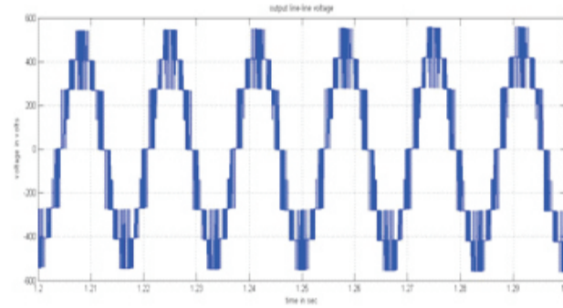
Fig.9. Output 9 level line to line voltage
