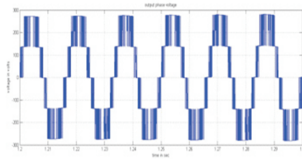
Fig.8. Output 5 level phase voltage
