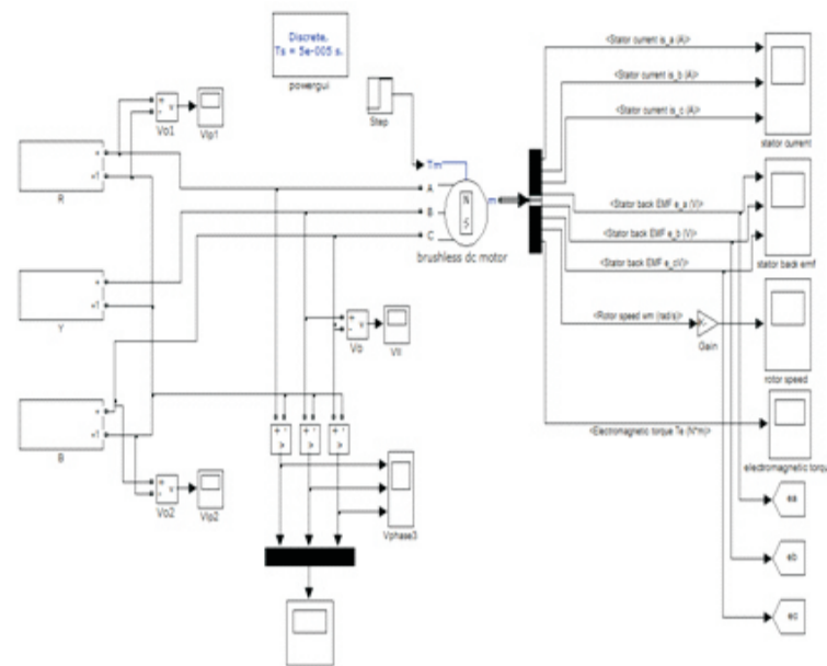
Fig.6. Simulink model of proposed Half Bridge power cells fed BLDC motor
