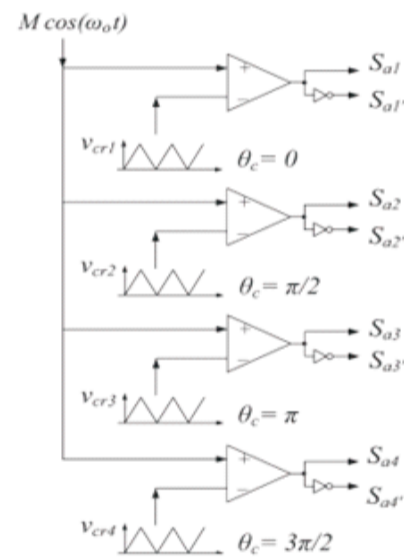
Fig.5. Simplified modulation schematic
