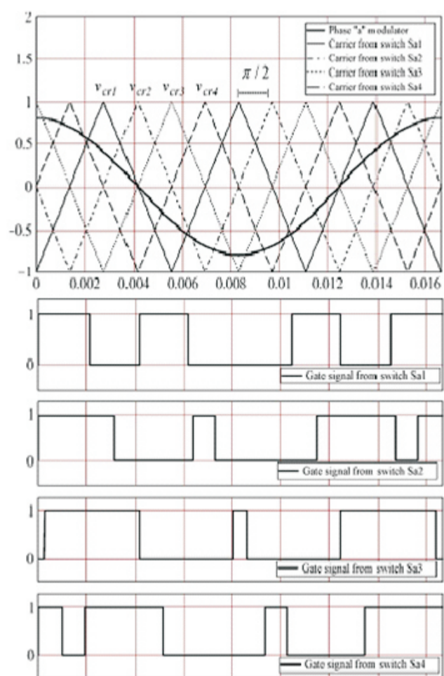
Fig.3. Simulated waveform of the proposed multilevel inverter
