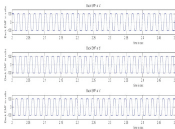
Fig. 12. Stator Back-EMF in each phase
