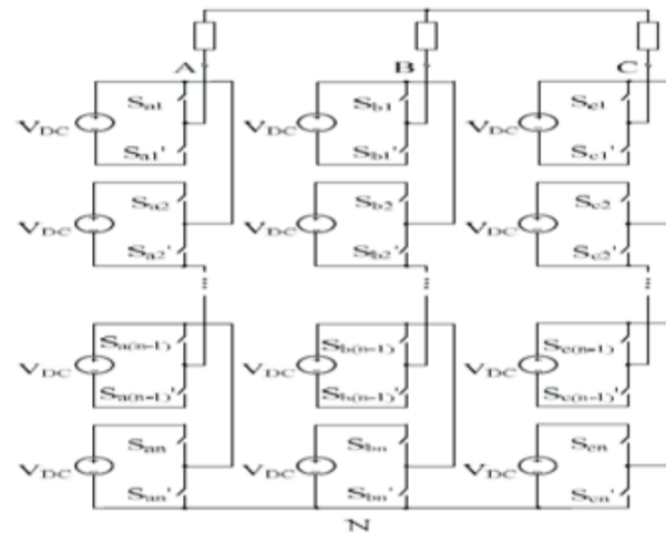
Fig.4. Multilevel inverter four inverter legs in cascade.
