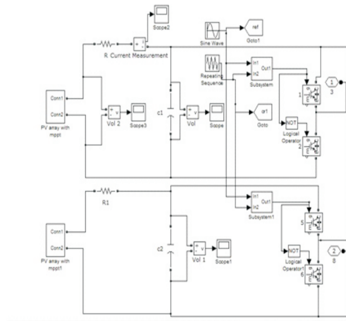
Fig. 7. Simulink diagram of PV array with MPPT connected as input
