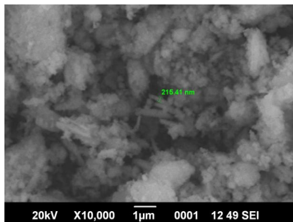
Figure.5 SEM image at 10000 magnifications.
