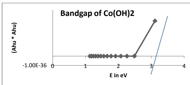
Figure.10 Graph to find the band gap of cobalt hydroxide nanoparticles.
