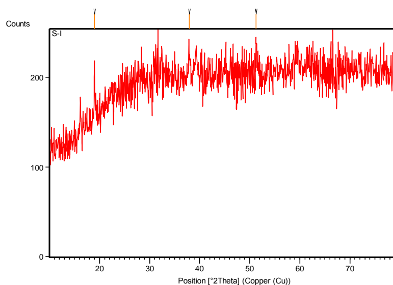
Figure.1 XRD pattern of cobalt hydroxide nano particles.
