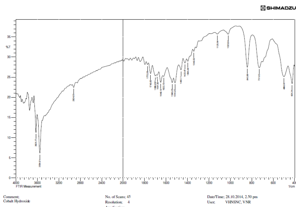
Figure.9 FTIR spectra of cobalt hydroxide nanoparticles.
