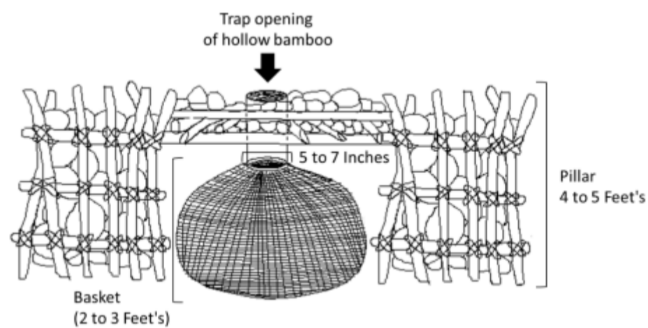
Figure 3. Construction of small 'Kuin' trap for small scale fishing (2 to 3 kg/day).
