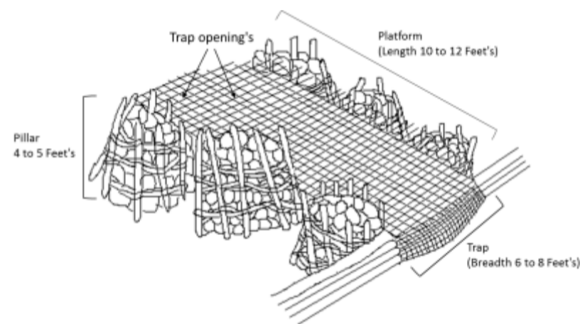
Figure 2. Construction of large 'Kuin' trap made for large scale fishing (3 to 10 kg/day).
